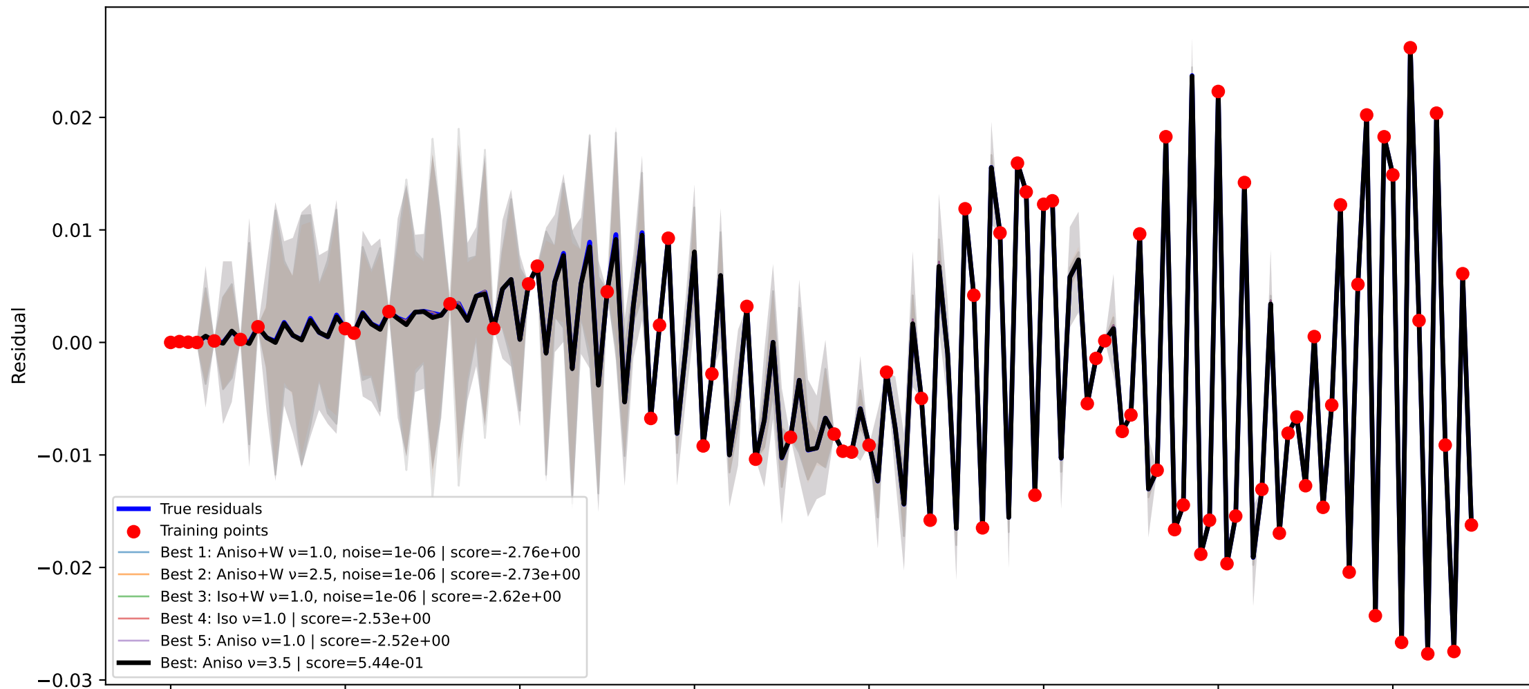
GPR kernel comparison node=25 RMSE=8.217e-05, train RMSE=1.628e-11
